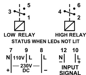
077 Terminal Diagram
